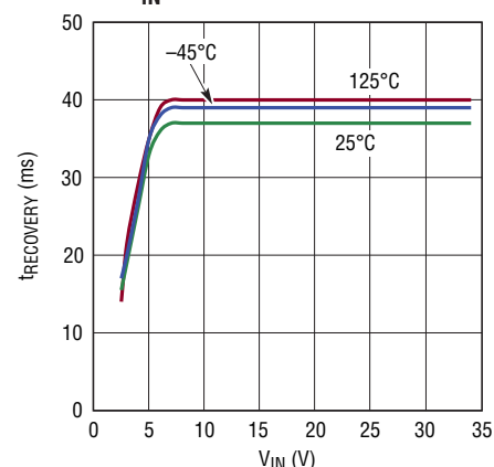
LTC4365 Recovery Delay Time vs V_IN
