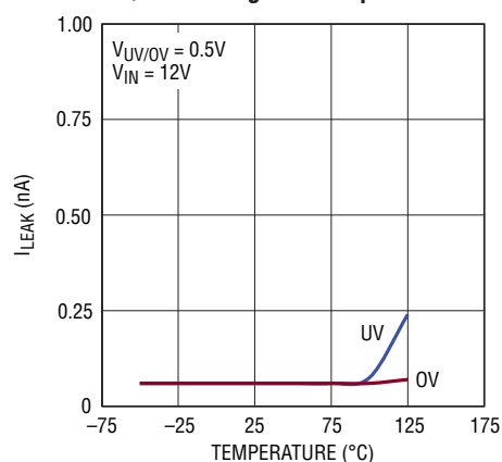
UV/OV Leakage vs Temperature
