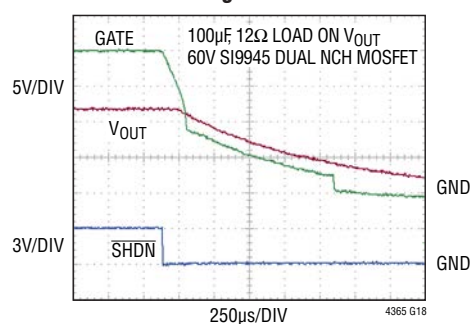
Turn-Off Timing
