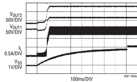
Start-Up Waveforms
