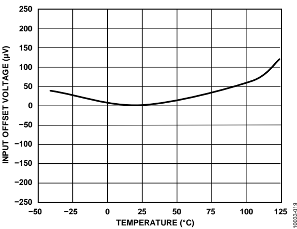
Figure 19. Output Buffer V_{OS} vs. Temperature
