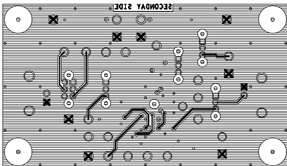
Figure 44. AD8436-EVALZ Secondary Side Copper
