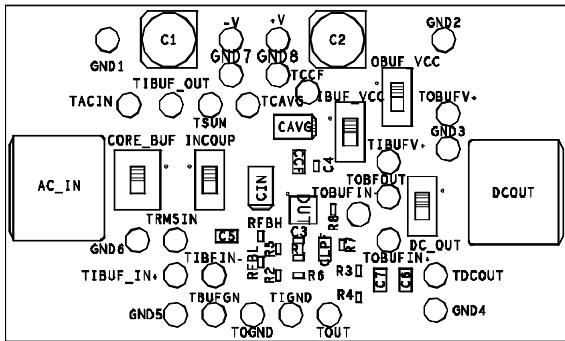
Figure 42. Assembly of the AD8436-EVALZ
