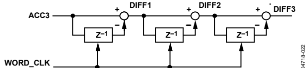
Figure 26. Differentiator
