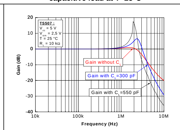
Figure 18. Closed loop gain in voltage follower configuration for different capacitive load at T=25^{\circ}C
