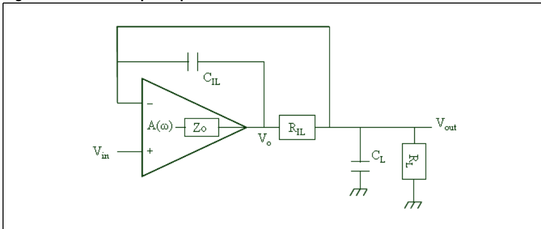
Figure 30. In-the-loop compensation schematics
