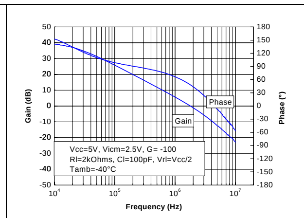
Figure 16. Voltage gain and phase vs. frequency at V_{CC}=5V and V_{icm}=2.5V at T=-40^{\circ}C
