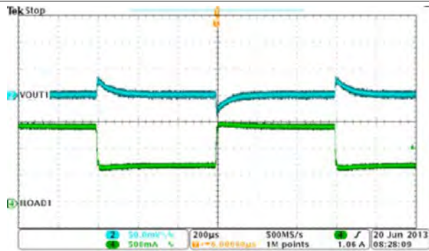
Figure 48. BUCK1, Load Transient, 0.75A to 1.5A SR=0.25A/µs
