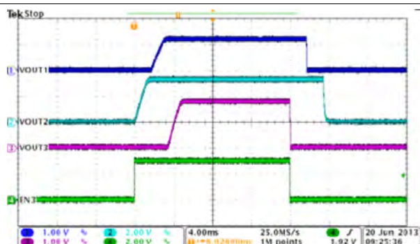
Figure 62. Automatic Power Sequencing, MODE=EN1= HIGH, EN2=LOW
