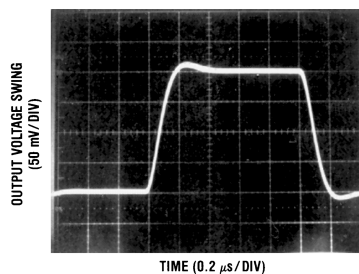
Figure 27. Small Signal Inverting
