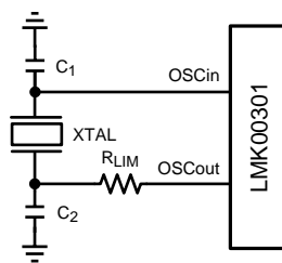
Figure 29. Crystal Interface
