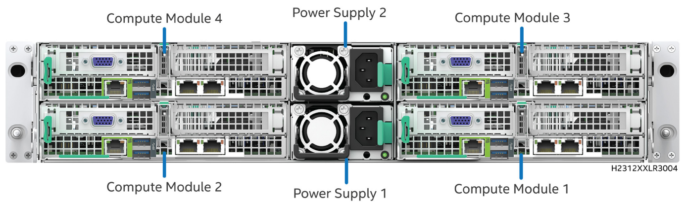
Figure 7. Intel® Server Chassis H2000G - Rear View
