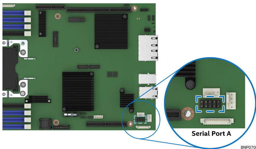
Figure 71. Serial Port A Location
