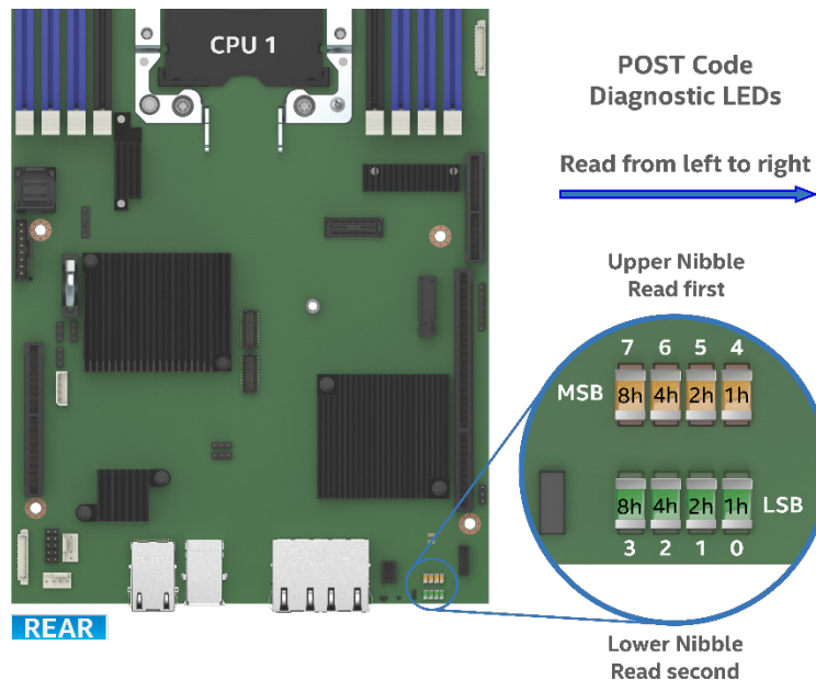
Figure 83. Rear Panel Diagnostic LEDs
