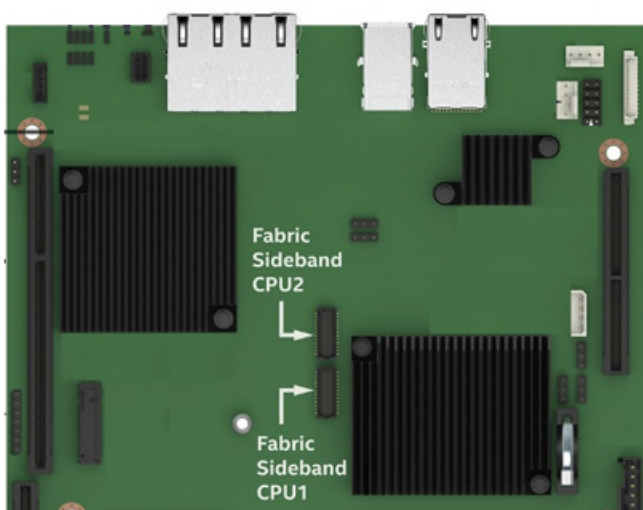
S2600BPB & S2600BPQ
