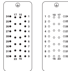
Connector pin assignment: Left pin - right socket
