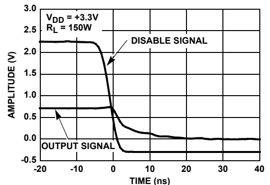
FIGURE 14. DISABLE TIME
