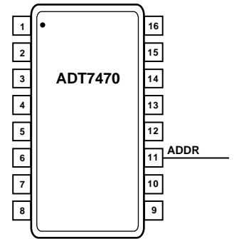
Figure 6. SMBus Address = 0x5C or 0x2E (Pin 11 = Floating)
