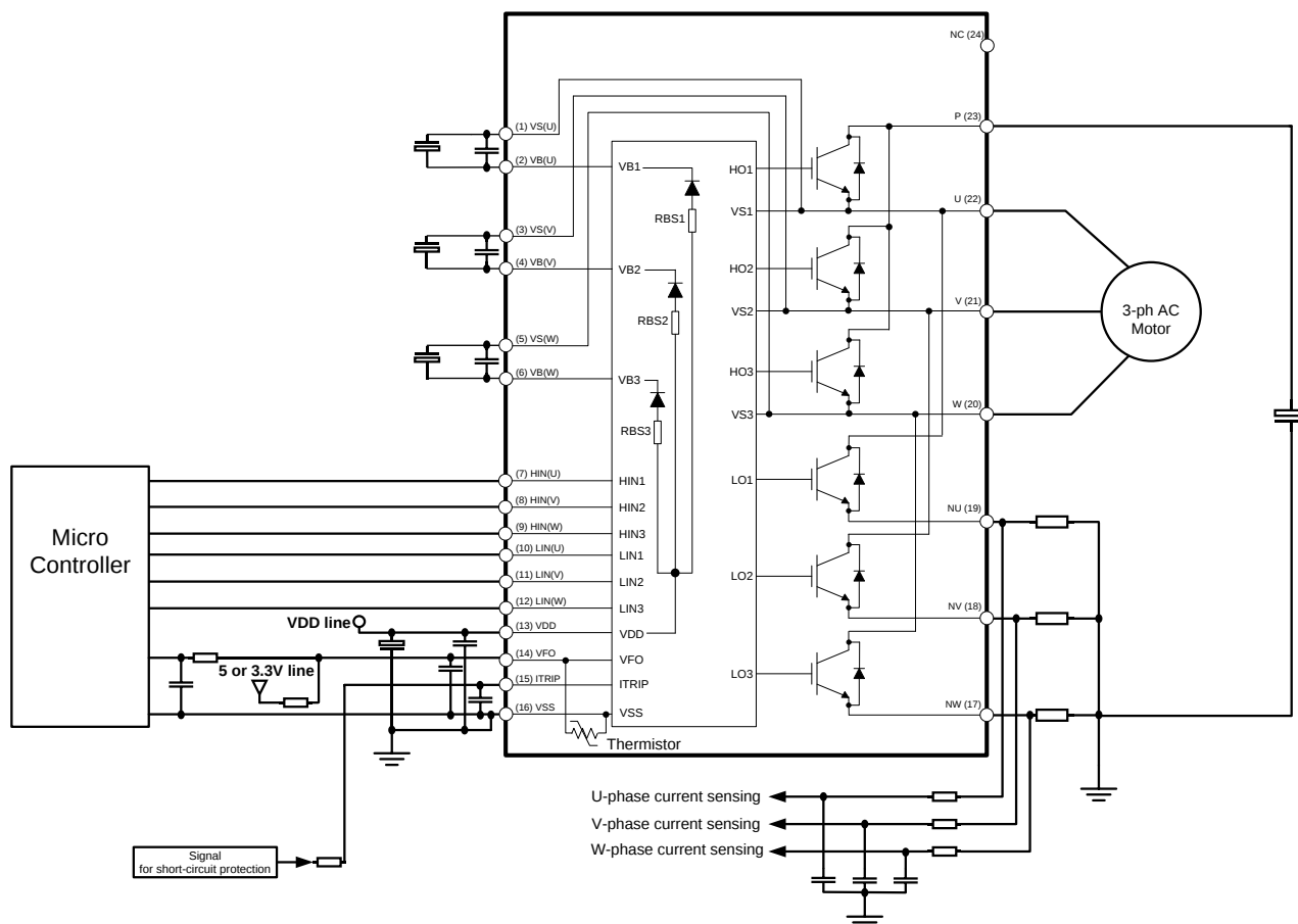
Figure 9: Application circuit
