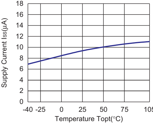
R1514x030B
