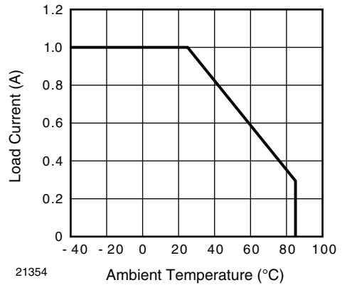
Fig. 2 - Allowable Load Current vs. Ambient Temperature
