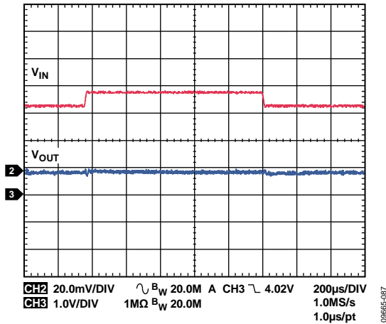
Figure 87. LDO1, LDO2 Response to Line Transient, Input Voltage from 3.3 V to 3.8 V, V_{OUT} = 1.8 V
