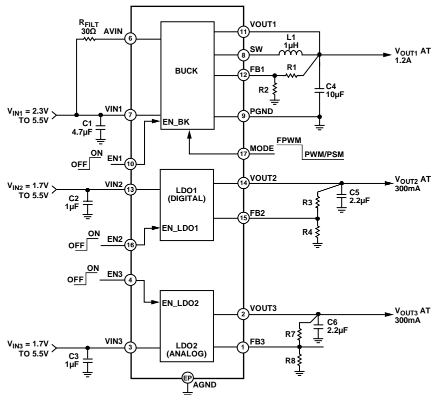
Figure 108. Application Diagram
