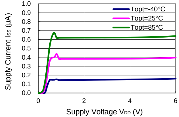
R3118xxxxA/C ( V_{SENSE}=6V )
