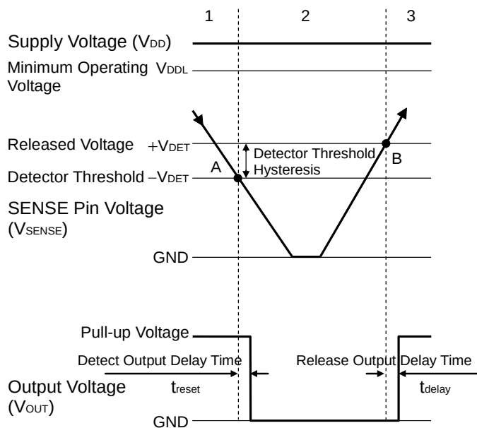
Operation Diagram
