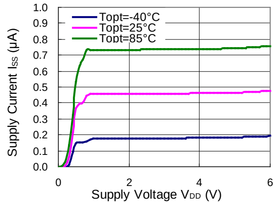
R3118xxxxA/C ( V_{SENSE}=0V )
