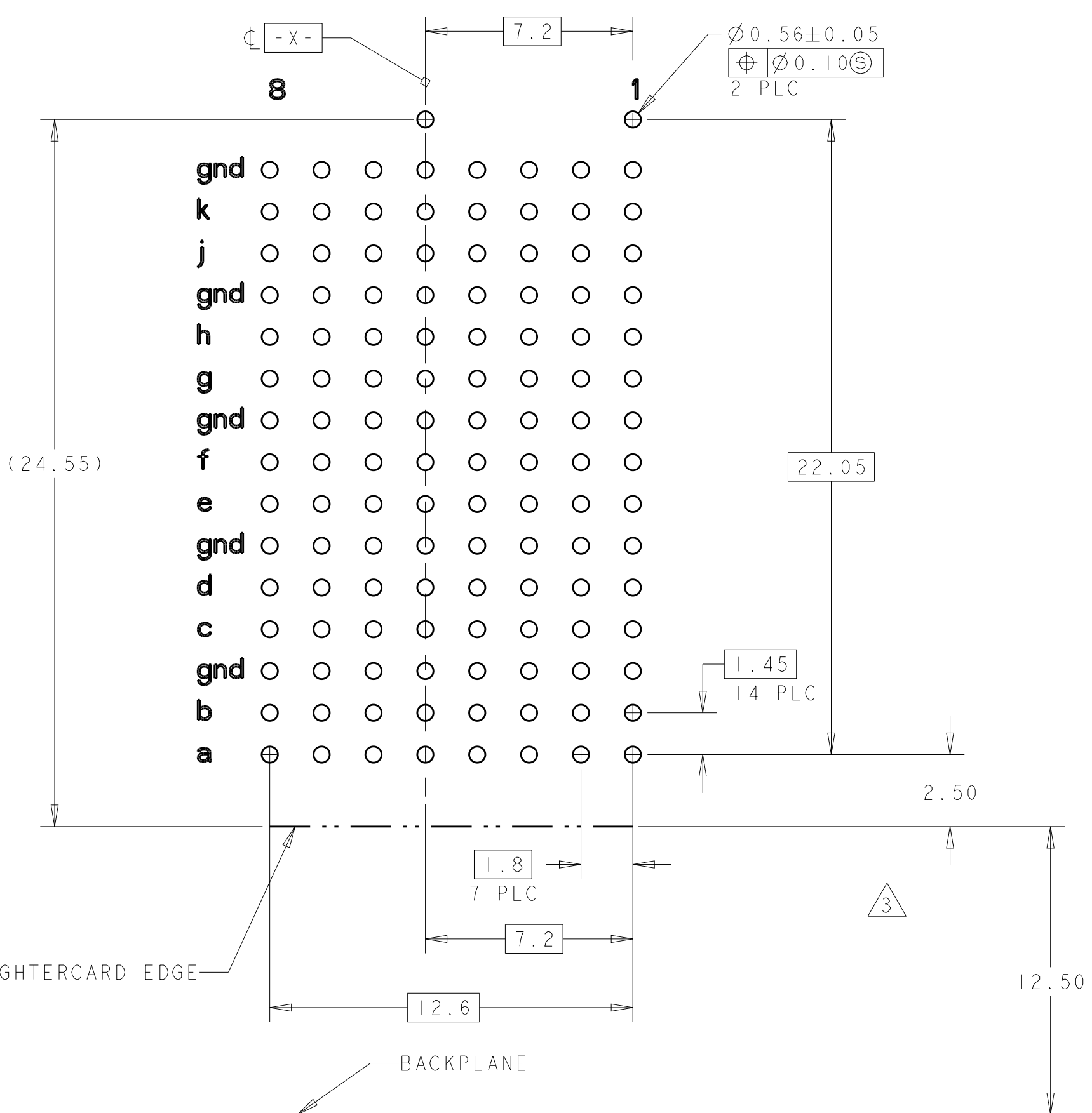
PCB LAYOUT (CONNECTOR SIDE) SCALE 6:1
