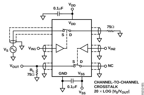
Figure 21. Channel-to-Channel Crosstalk
