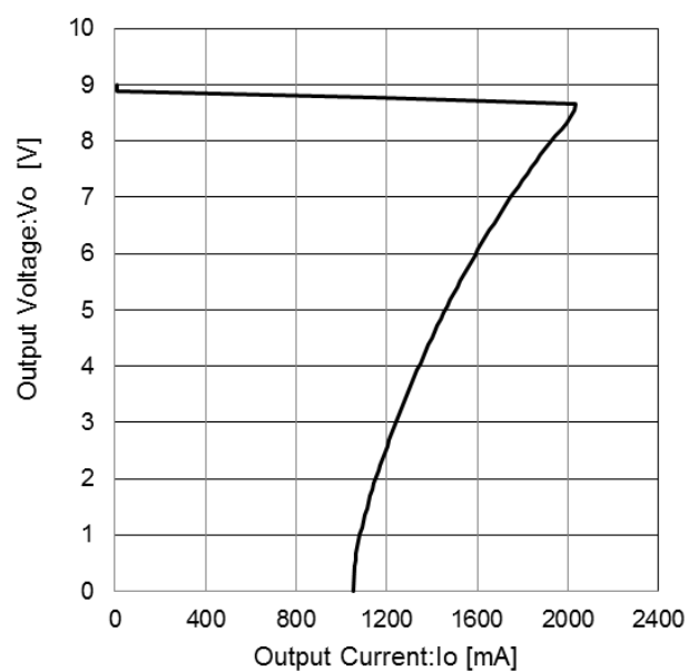
Figure 16. Load Regulation
