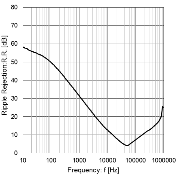
Figure 18. Ripple Rejection ( I_o=100mA )
