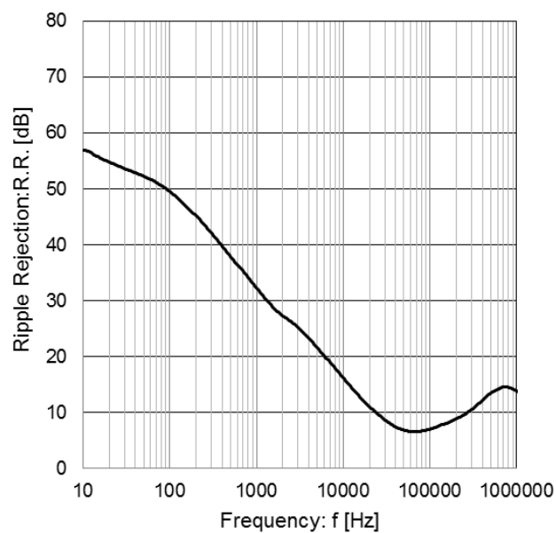
Figure 9. Ripple Rejection (I_o = 100mA)
