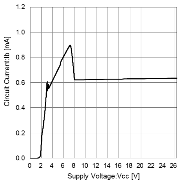
Figure 4. Circuit Current
