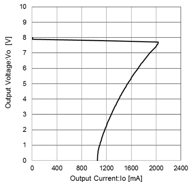
Figure 7. Load Regulation
