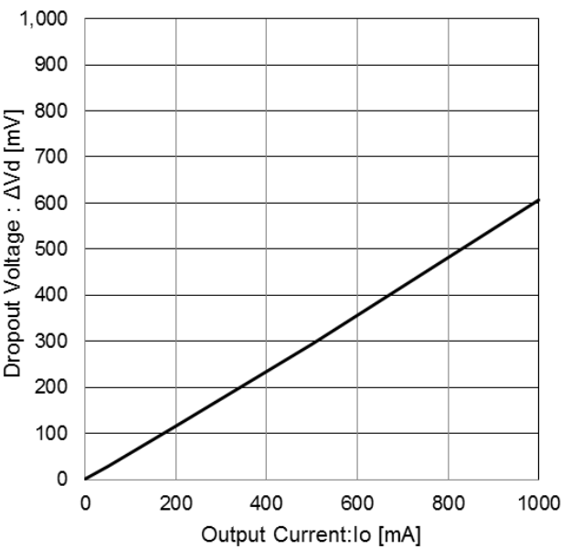
Figure 17. Dropout Voltage ( V_{cc}=V_o \times 0.95V ) ( I_o=0mA \rightarrow 1000mA )
