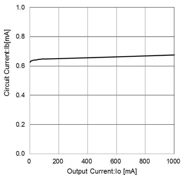
Figure 11. Circuit Current (I_o=0mA \rightarrow 1000\text{ mA})
