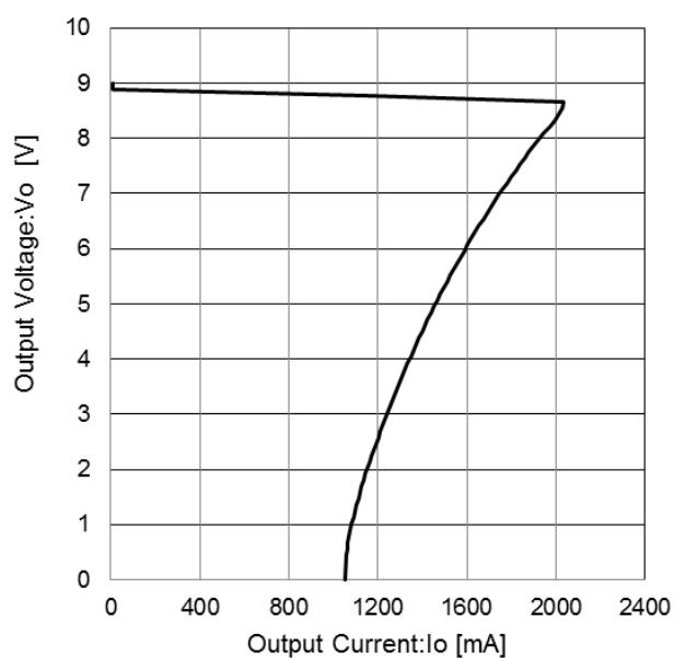
Figure 16. Load Regulation
