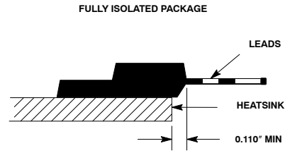
Figure 3. Mounting Position
