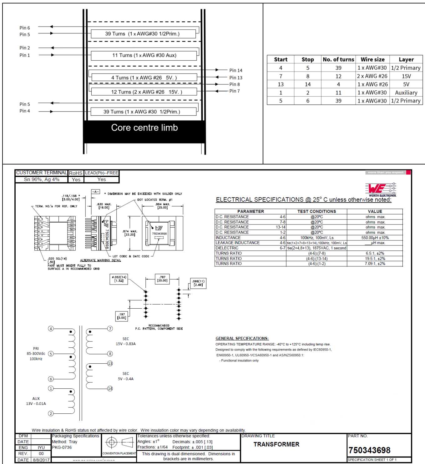
Figure 6 Transformer structure
