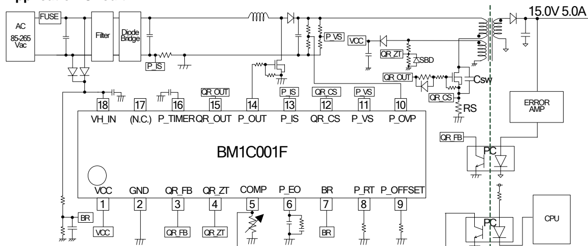
Figure 1. Application circuit
