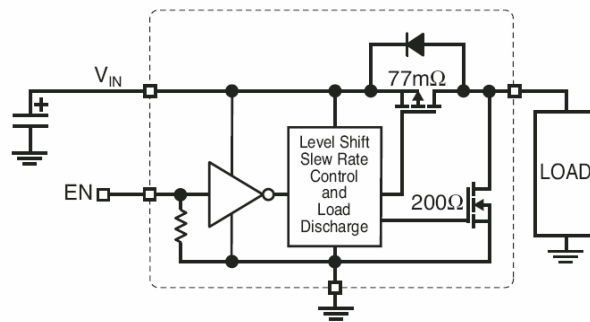
MIC94065 Load Switch with Capacitive Load Discharge
