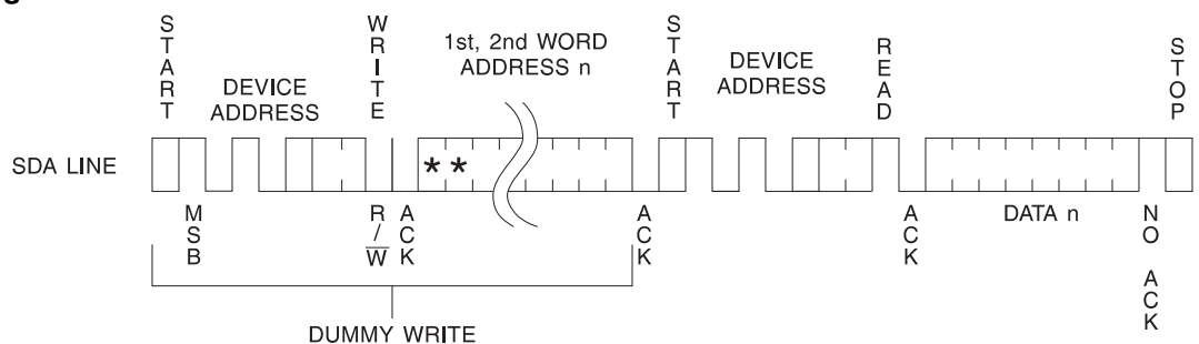
Figure 9-2. Random Read
