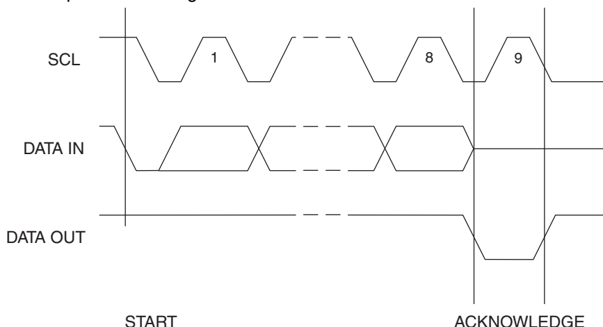
Figure 6-6. Output Acknowledge
