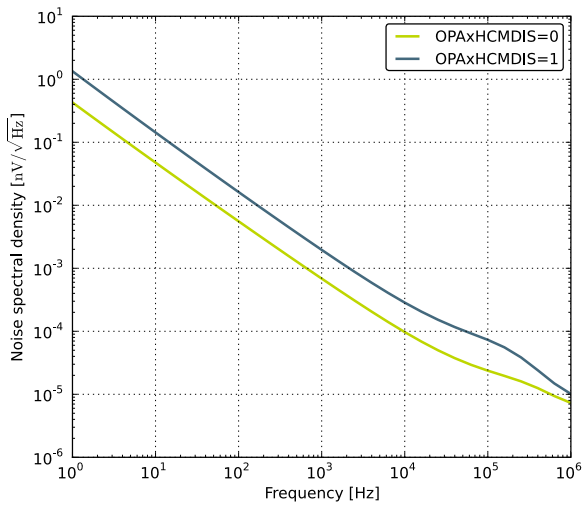
Figure 3.40. OPAMP Voltage Noise Spectral Density (Non-Unity Gain)
