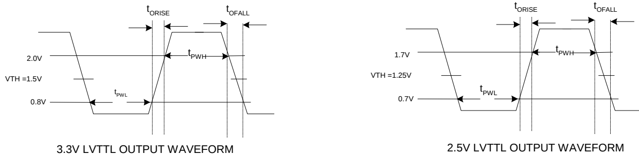
Figure 3. Output Waveforms
