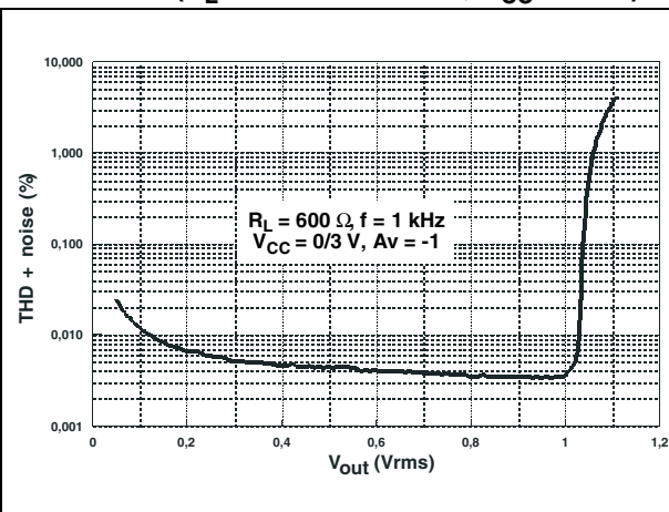
Figure 10. THD + noise vs. output voltage (R_L = 600\ \Omega, f = 1\ kHz, V_{CC} = 0/3\ V)
