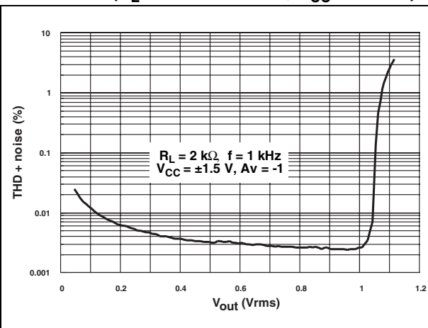
Figure 12. THD + noise vs. output voltage (R_L = 2\ k\Omega, f = 1\ kHz, V_{CC} = \pm 1.5\ V)
