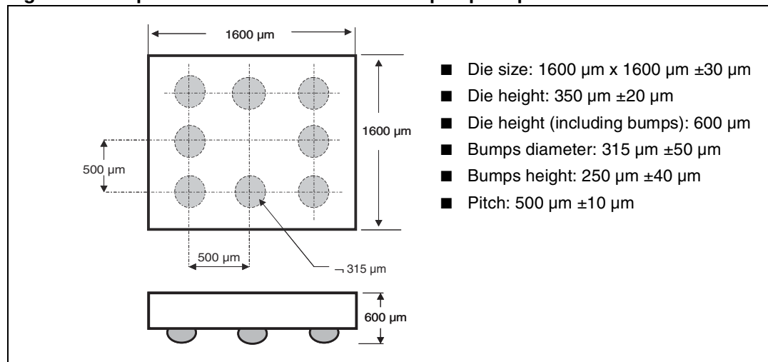
Figure 14. Top view and dimensions of 8-bump Flip-Chip
