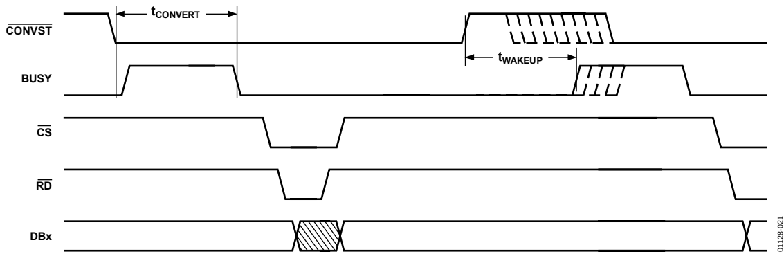
Figure 21. Mode 2 Operation
