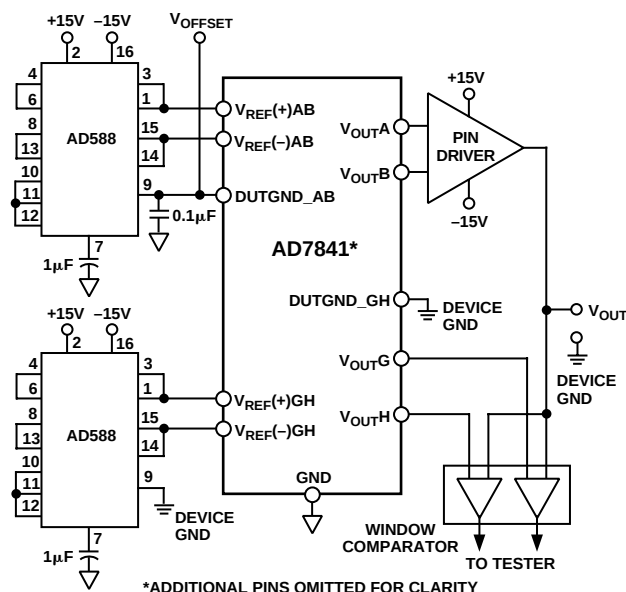
Figure 21. ATE Application
