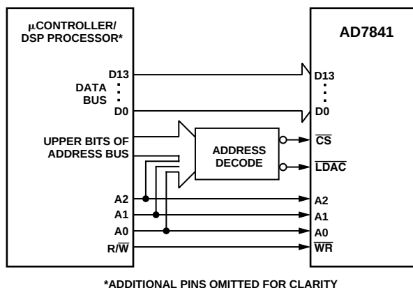
Figure 19. AD7841 Parallel Interface
