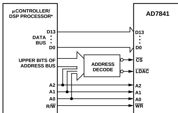
Figure 19. AD7841 Parallel Interface
