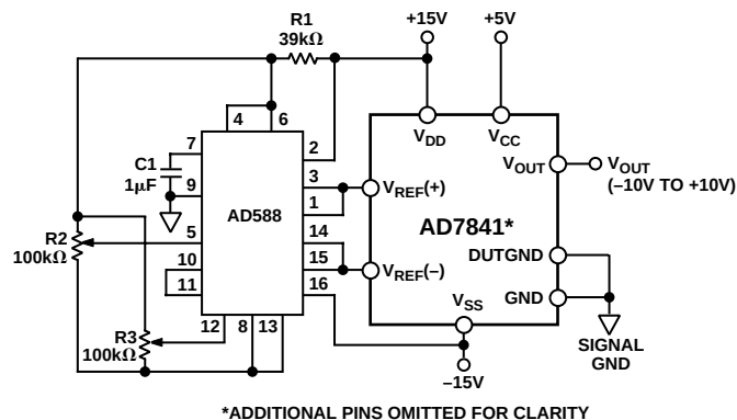
Figure 12. Bipolar \pm 10 V Operation
