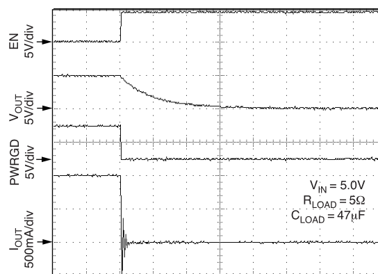
5V Turn-Off
