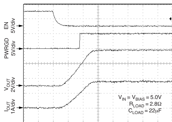
5V Turn-On
