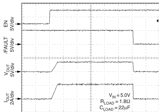
Latched Output (MIC2043)
