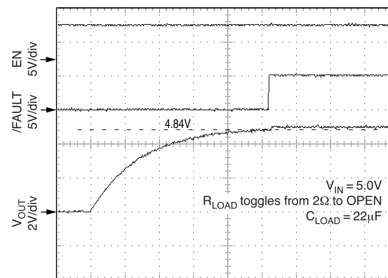
Latched Output Reset (MIC2043)
