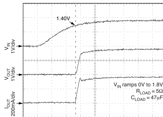
UVLO Response
