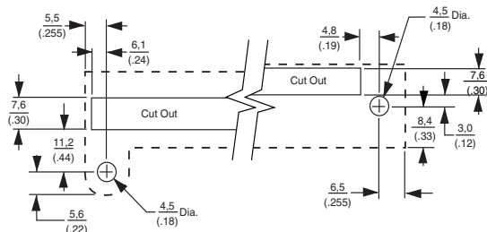
VERTICAL MOUNTING PANEL LAYOUT
