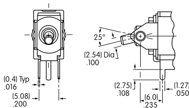
Vertical PC Mounting
