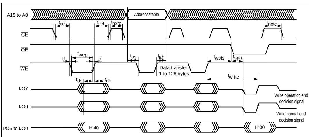
Figure 6.17 Timing Waveforms in Auto-Program Mode
