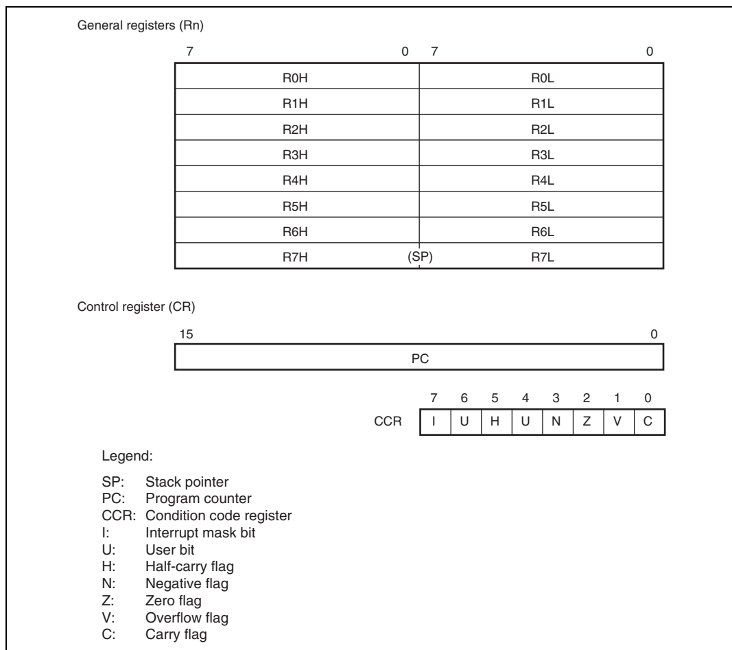
Figure 2.2 CPU Registers
