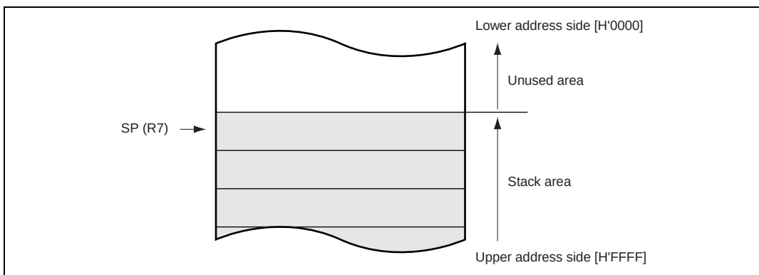
Figure 2.3 Stack Pointer
