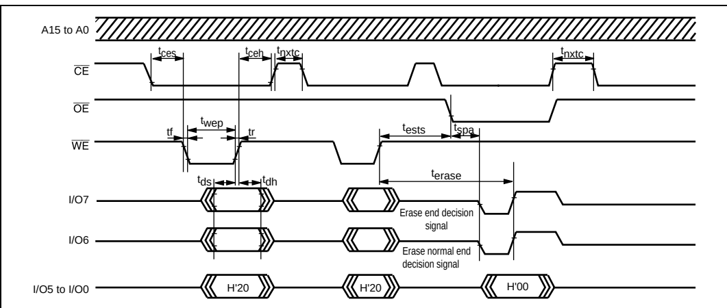
Figure 6.18 Timing Waveforms in Auto-Erase Mode
