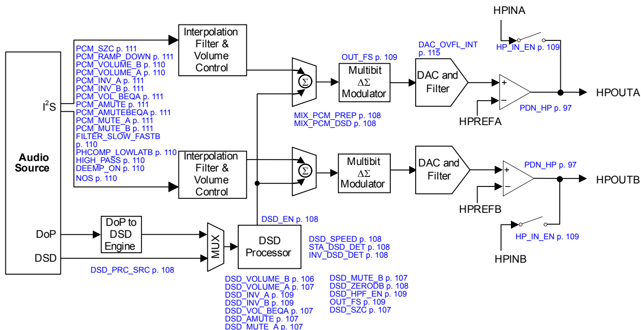
The CS43130 has 4 settings of full scale voltage, which are determined by OUT_FS[1:0]. The proper full scale voltage must be set first, and the digital volume settings is used to control signal levels.
