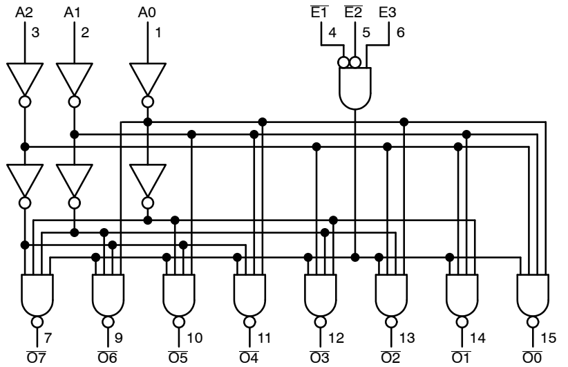
Figure 2. Logic Diagram
