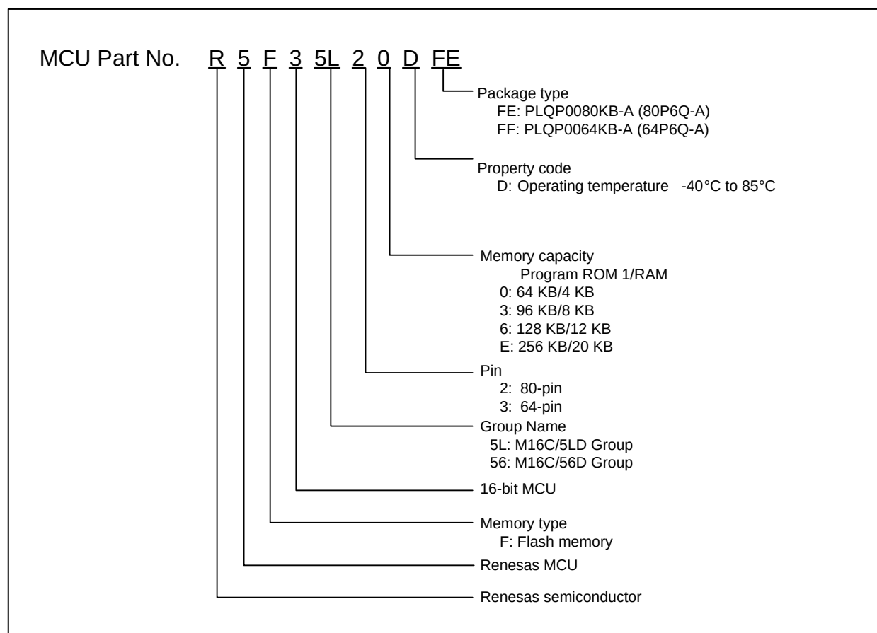
Figure 1.1 Correspondence of Part Number, Memory Size, and Package
