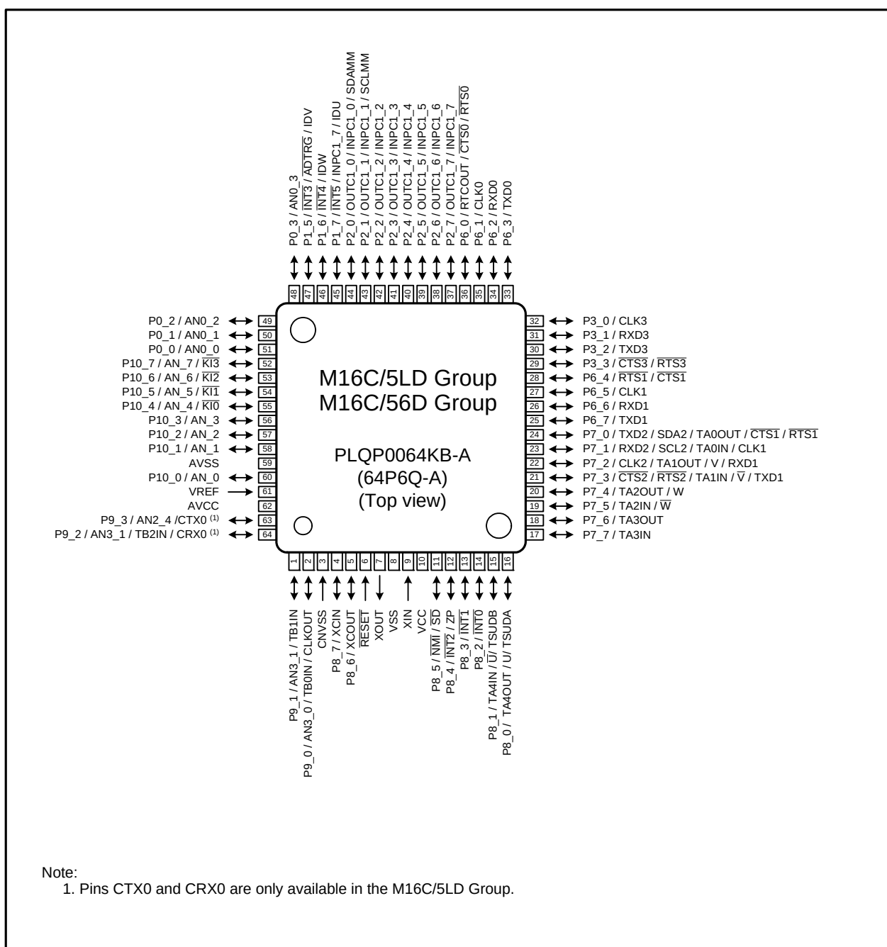
Figure 1.6 Pin Assignment for 64-Pin Package (Top View)
