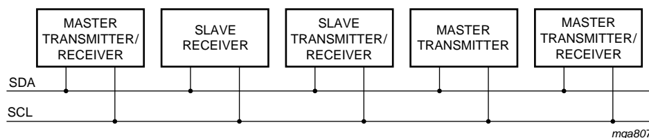
Fig 15. System configuration
