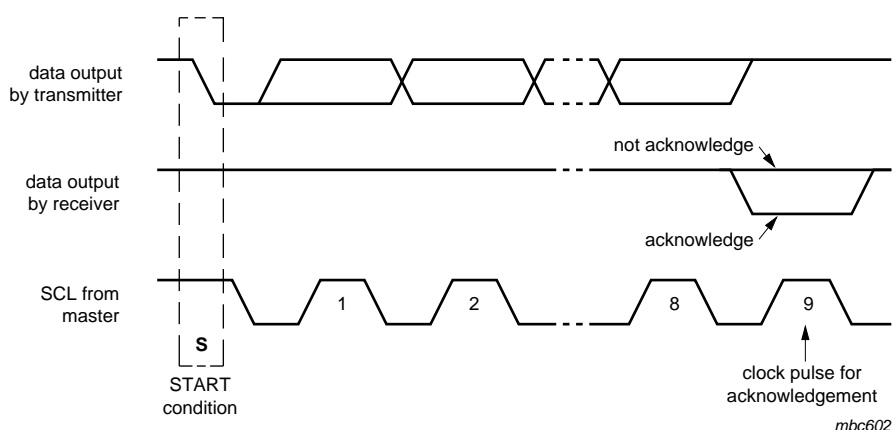
Fig 16. Acknowledgement of the I 2 C-bus
