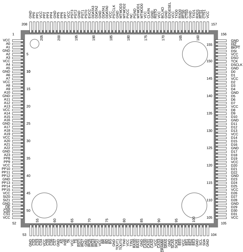
Figure 16-1. Mechanical Diagram
