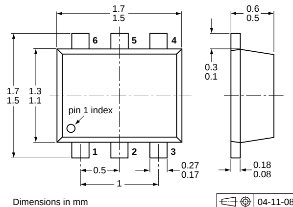
Fig 14. Package outline SOT666
