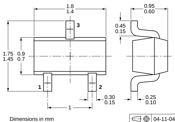
Fig 13. Package outline SOT416 (SC-75)
