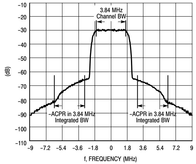
Figure 19. Single-Carrier W-CDMA Spectrum
