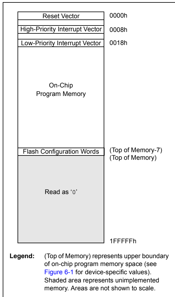
FIGURE 6-2: HARD VECTOR AND CONFIGURATION WORD LOCATIONS FOR PIC18F87J11 FAMILY DEVICES
