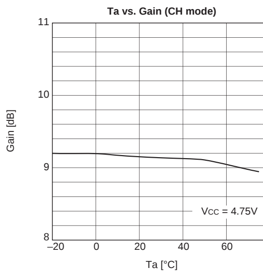
CH mode AMP gain temperature characteristics
