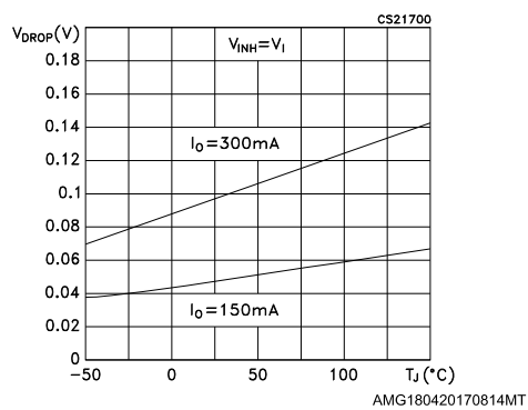
Figure 15: Dropout voltage vs temperature
