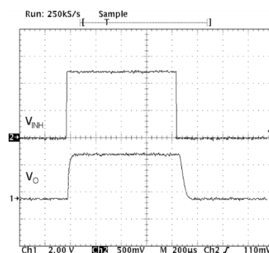
Figure 17: Inhibit transient
