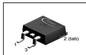
PG-TO263-3
