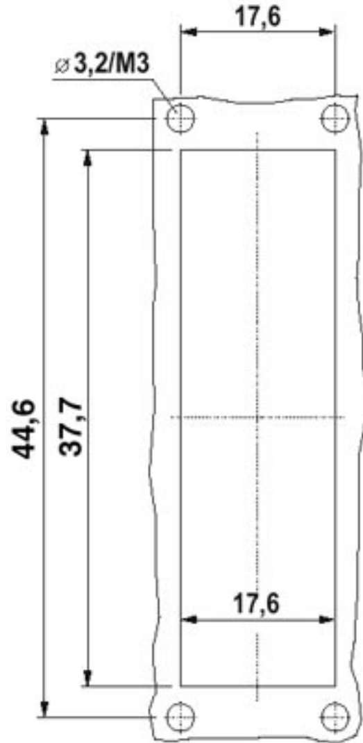
Dimensioned drawing
